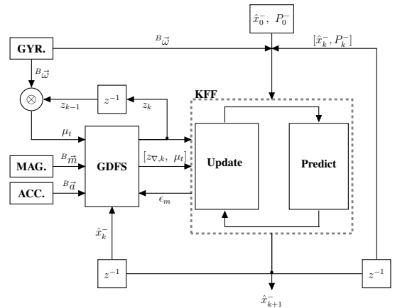
Fig. 2. Diagram of both filter stages, the Kalman filter framework (KFF) and the gradient descent filter stage (GDFS), and their interconnections [8].
