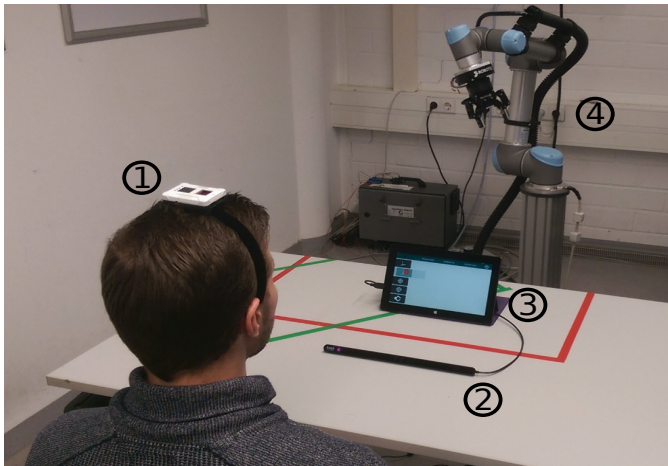
Fig. 4. Setup for the proposed hybrid MARG and visual interface. The user is seated in front of the Tobii eye tracker (2) while the XDK 110 (1) is placed on the user's head by a headband. Data from the hybrid system is fed to the computer (3) to calculate orientation and control a robotic arm (4, UR5).
