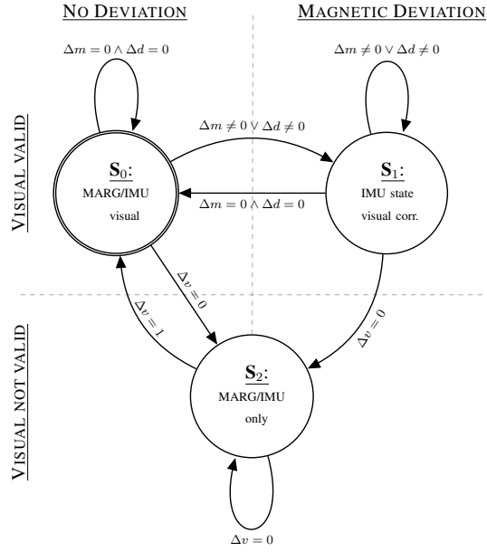
Fig. 3. State Machine SM \{\Sigma, S_0, S_1, S_2, \delta\} .
