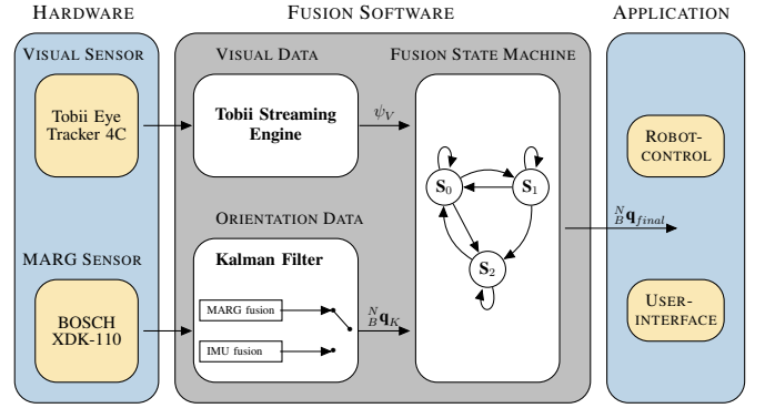
Fig. 1. General concept of the proposed fusion method.
